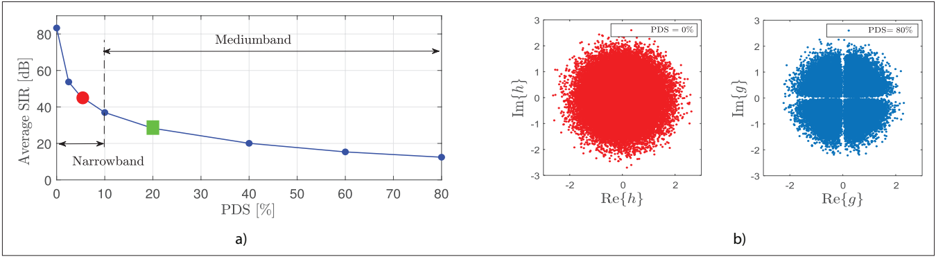
FIGURE 4. a) Typical trend of average SIR with PDS. When PDS is less than 10 %, the narrowband model in Eq. 2 is deemed to be satisfied, and the larger region, where PDS is greater than 10 %, is the mediumband region. The RED circle (i.e., PDS = 5%) represents a narrowband system, while the GREEN square (i.e., PDS = 20%) represents a mediumband system [1]; b) Scatter plots showing the real and imaginary parts of h in Eq. 2 and g in Eq. 4 in NLoS propagation, where \beta = 0.22 and N = 10 (see Table 1 for variable definitions). The low correlation between the real and the imaginary dimensions and, due to the “four leaf clover” shape the effect of deep fading avoidance in g are clearly visible.
