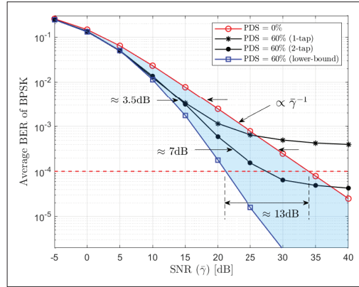
FIGURE 8. Average BER of BPSK modulation against the received SNR \bar{\gamma} for PDS = 60 % in NLoS propagation. The lower bound is from [27, eq. 16] with values for K , \sigma_f^2 and \sigma_0^2 from Table 2.
