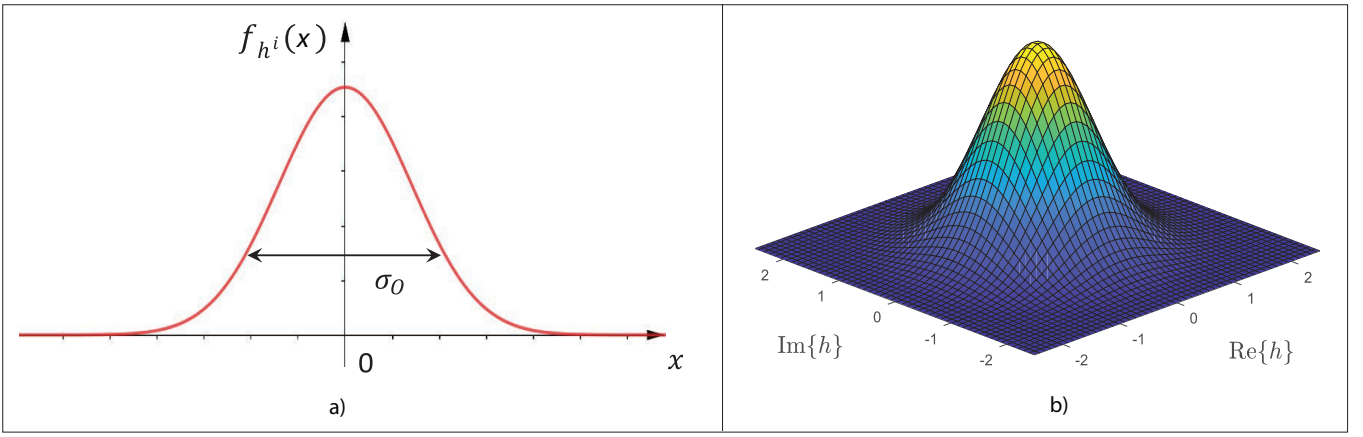
FIGURE 3. a) A graphical depiction of the PDF of h in a typical NLoS propagation environment as described in Eq. 3. Typically, h is complex, but here only the PDF of the real part of h denoted by h^i , that is f_{h^i}(x) , is shown for brevity. Note that \sigma_0 is a parameter to capture the width of the PDF, but does not measure the distance as shown; b) A depiction of f_{h^i}(x, y) = f_{h^i}(x)f_{h^i}(y) , which is the complex PDF of h . Note the peak at (0, 0) signifying the fact that the probability of either \text{Re}\{h\} or \text{Im}\{h\} being very small is very high, which is the single most problematic dampening force in modern wireless communication.
