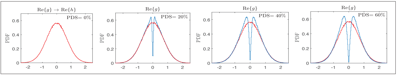
FIGURE 9. The evolution of the hole behavior in the marginal PDF of g (i.e., of \text{Re}\{g\} and \text{Im}\{g\} ) as PDS increases. This is from 1 million samples each from a detailed link-level simulation using the parameters in Table 1.
