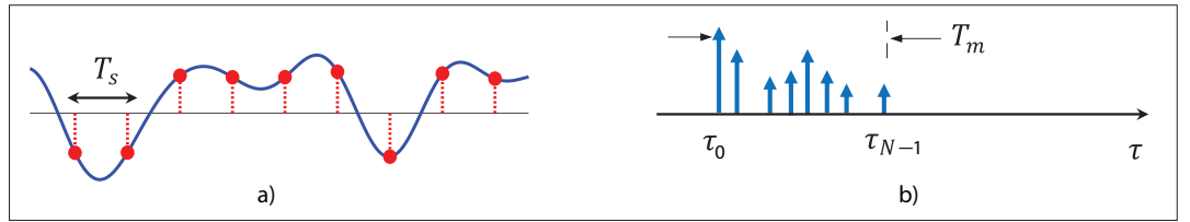
FIGURE 2. a) A depiction of a typical transmit signal s(t) . In digital wireless communication, not all parts of s(t) , but only the points regularly separated in time (i.e., RED dots), carry information. This separation time is the symbol period or T_s ; b) A depiction of a multipath delay profile as an impulse train, where the x -coordinate and the height of the impulse represent the excess delay and the strength of the corresponding MPC respectively. T_m is a suitable measure of the time spread of MPCs. A wireless communication system, whose T_m and T_s approximately satisfy the condition: 0.1T_s \leq T_m \leq T_s , which is represented by the GREEN region in Fig. 1, is said to be operating in the mediumband.
