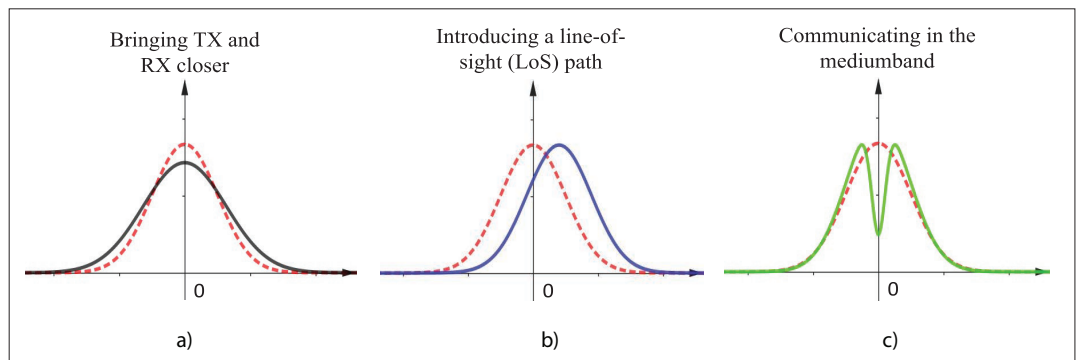
FIGURE 6. Depictions of the resulting PDFs (only a single dimension) of the desired fading factor in several methods known to reduce deep fading.
