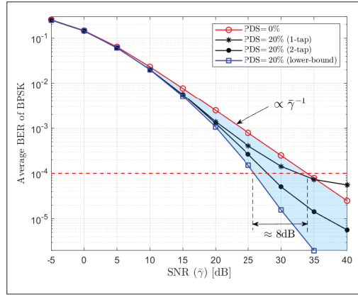
FIGURE 7. Average BER of BPSK modulation against the received SNR \bar{\gamma} for PDS = 20 % in NLoS propagation. The lower bound is from [27, eq. 16] with values for K , \sigma_f^2 and \sigma_0^2 from Table 2.
