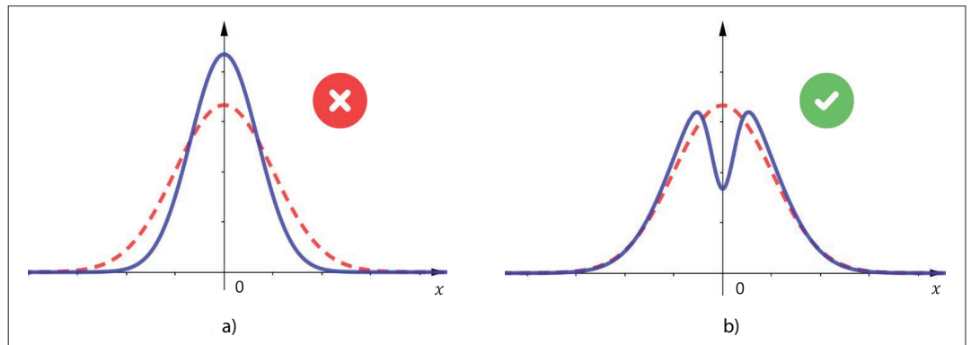
FIGURE 5. On the right is the typical PDF of g (only the real part) in a typical NLoS propagation environment [1, 2]. Importantly, it is the same NLoS environment, which gives rise to the Gaussian PDF (in RED dotted line) for h for narrowband systems, that gives rise to the bimodal PDF (in BLUE solid line) for g for mediumband systems. It is the different operating points on the T_m T_s -plane that create this difference, but not different propagation environments.
