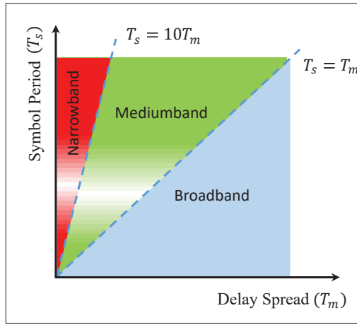
FIGURE 1. Main regions on the T_m T_s -plane representing three classes of wireless channels [1].
